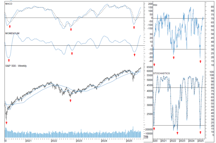
Figure 3: S&P 500
