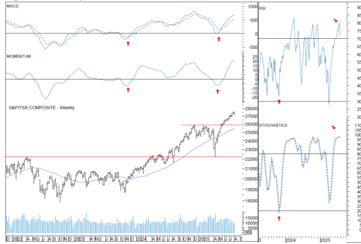
Figure 2: S&P/TSX
